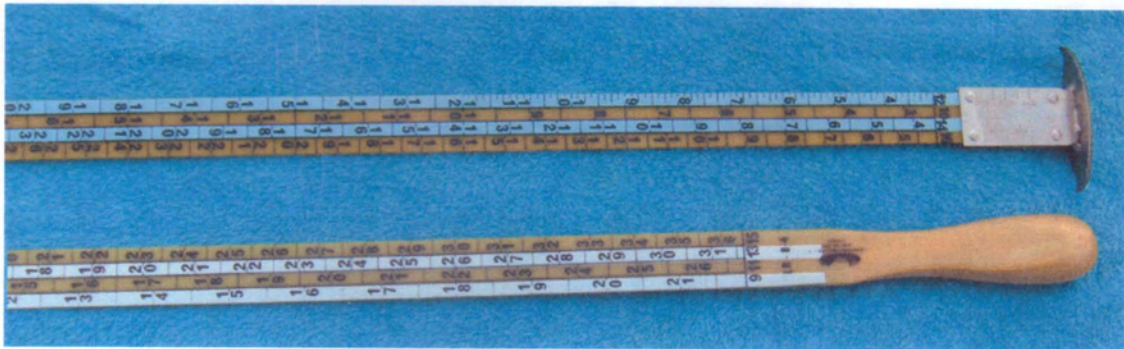
Board Volume in Board Feet (8'-16' Planks)
