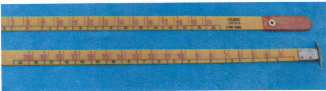
20" , 8ft Rough Imperial Pulp Ruler
